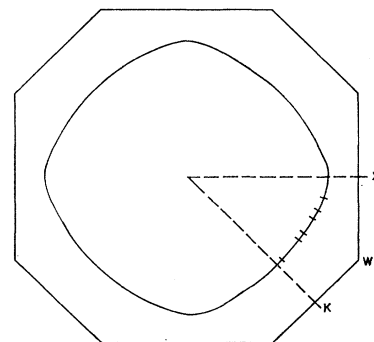
FIG. 7. (100) cross-section of the Fermi surface.
